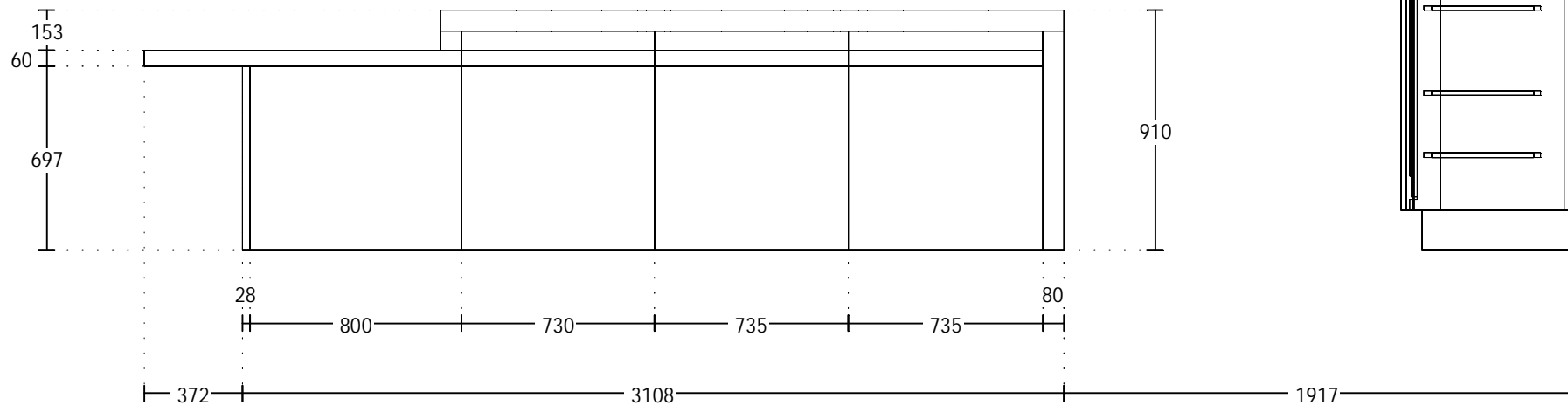
ELEVATION D
