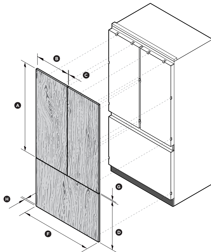
ISO VIEW
