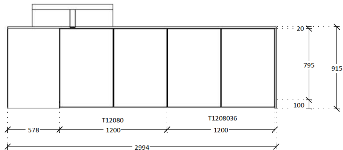
ELEVATION C
