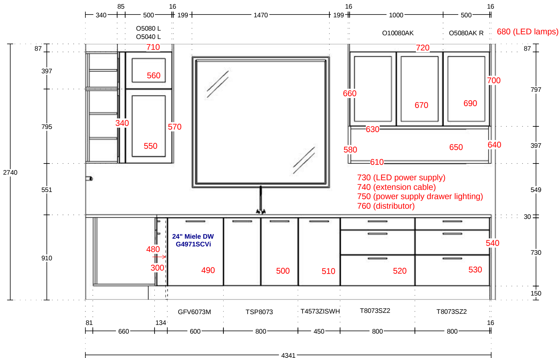
ELEVATION C
