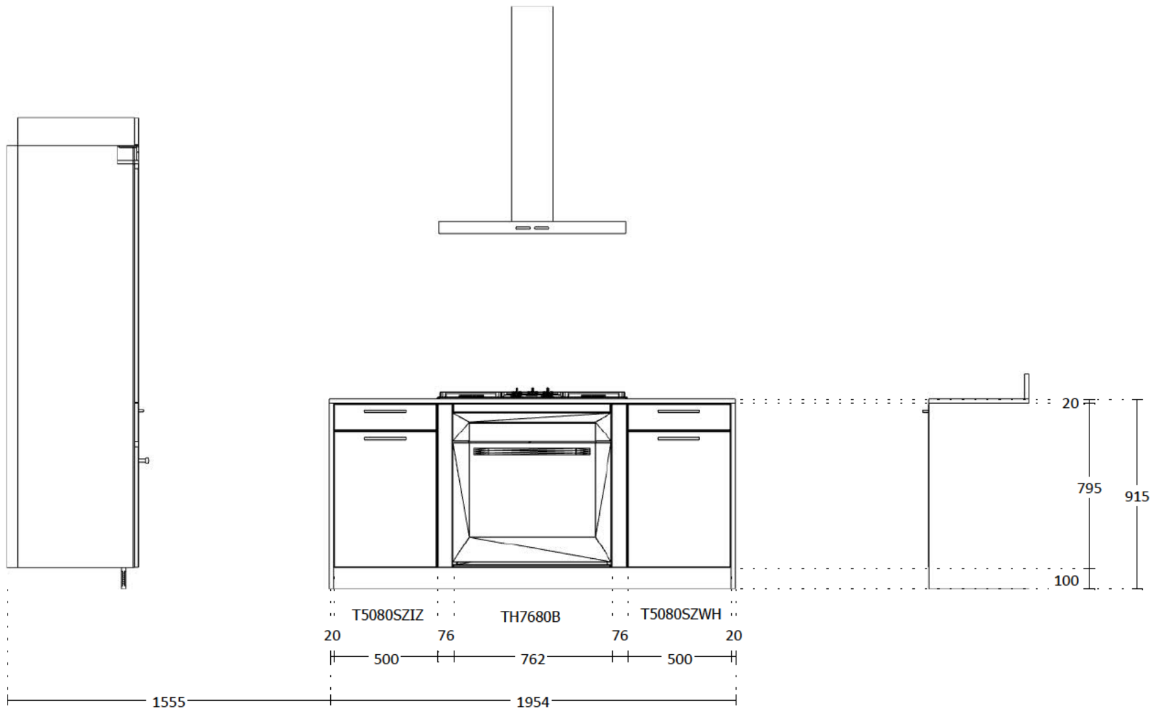
ELEVATION C
