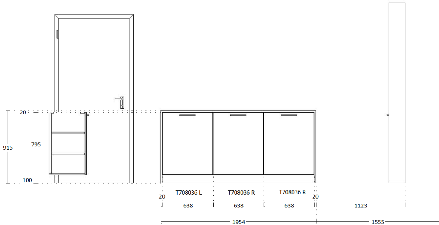
ELEVATION D
