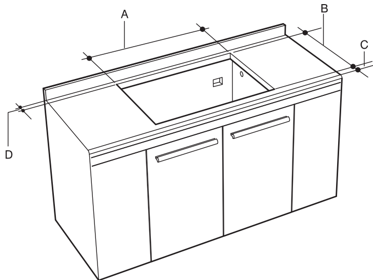
Figure 8. Cutout Requirements (1/2)
