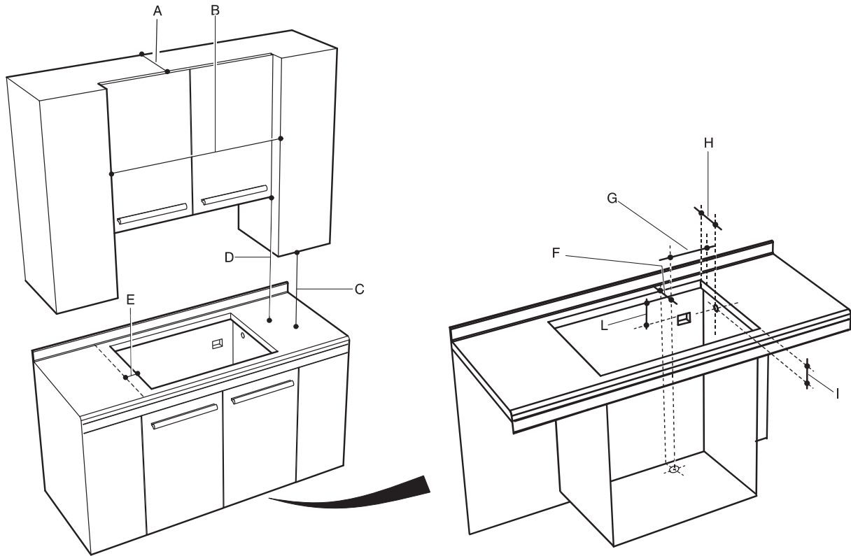
Figure 9. Cutout Requirements (2/2)
