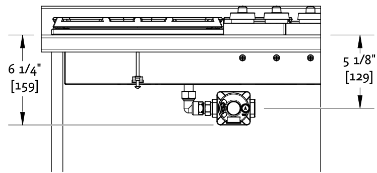
Figure 6. Regulator clearance
