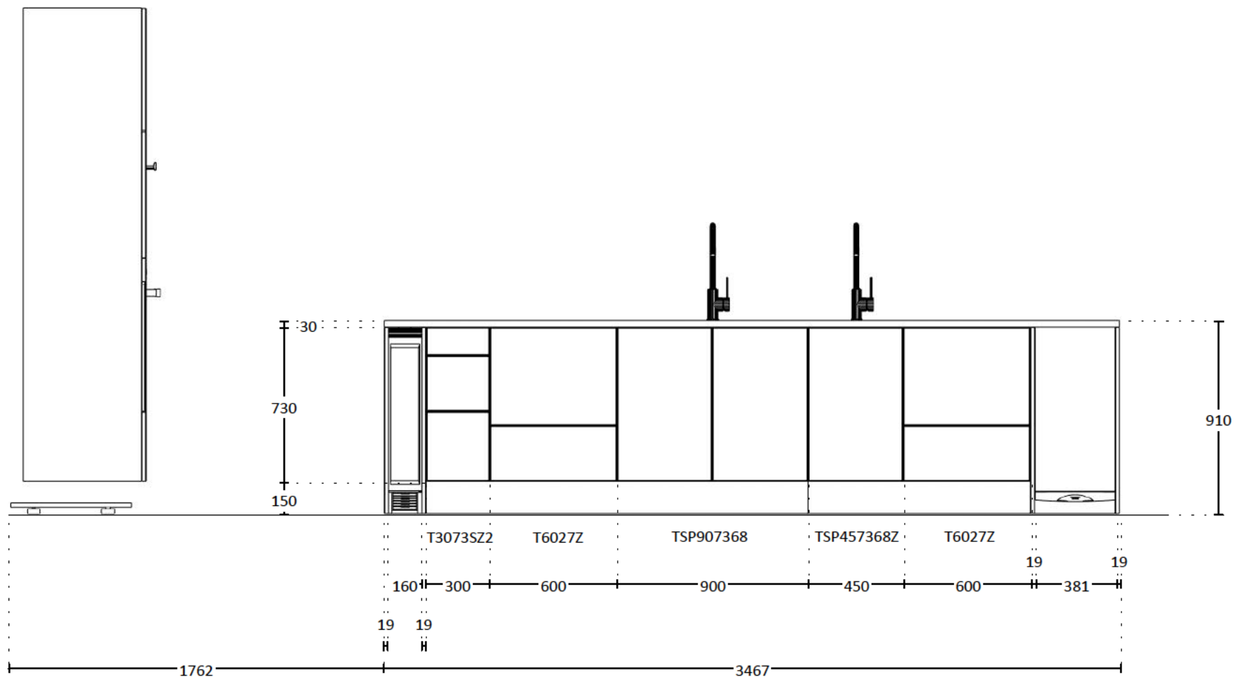
ELEVATION C
