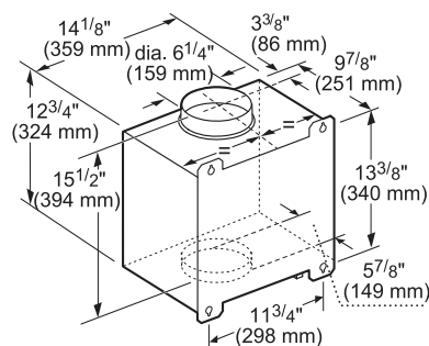
DHG6015NUC 600 CFM Inline Blower
