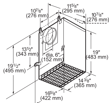
DHG6023RUC 600 CFM Remote Blower
