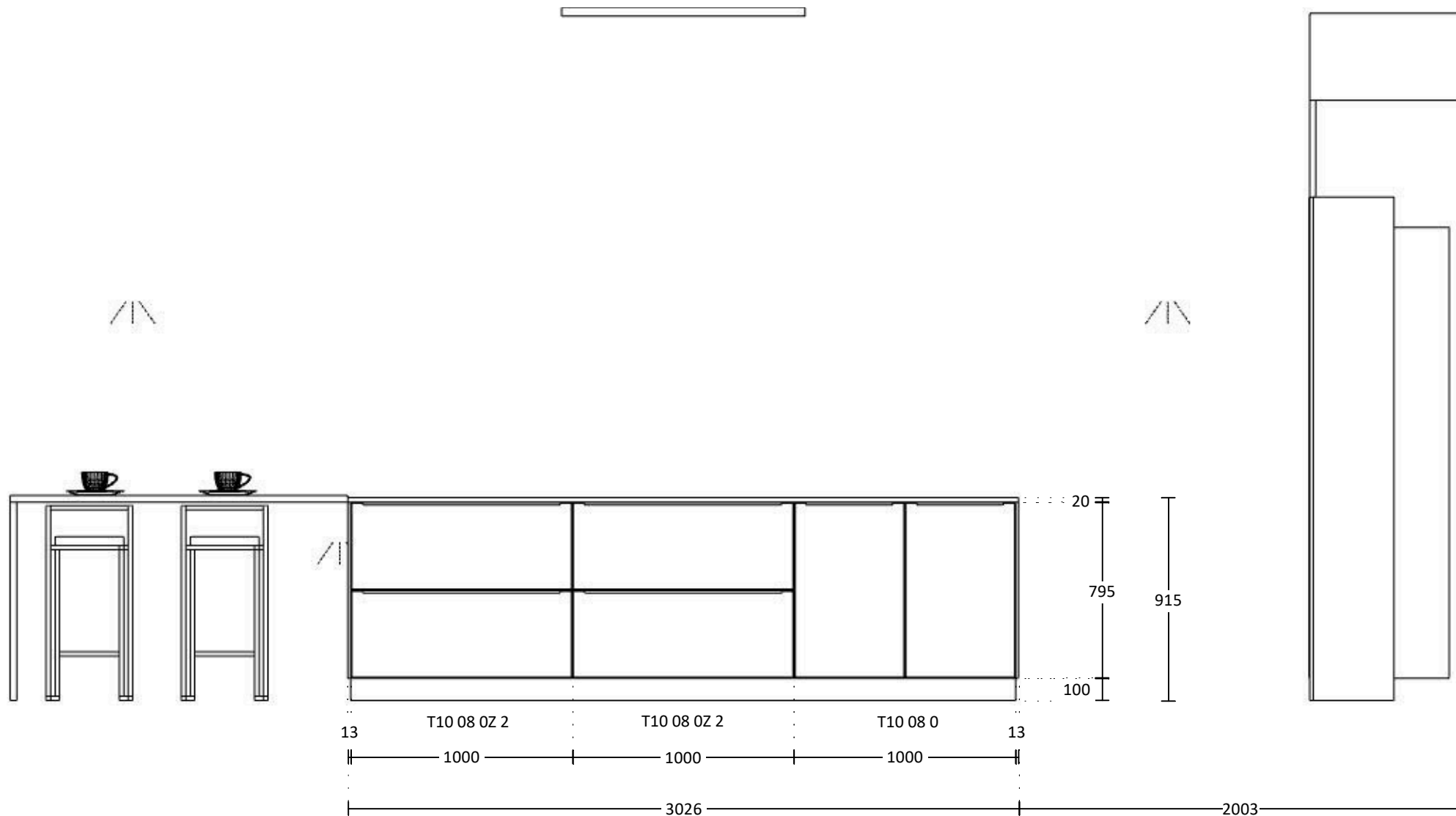
ELEVATION C
