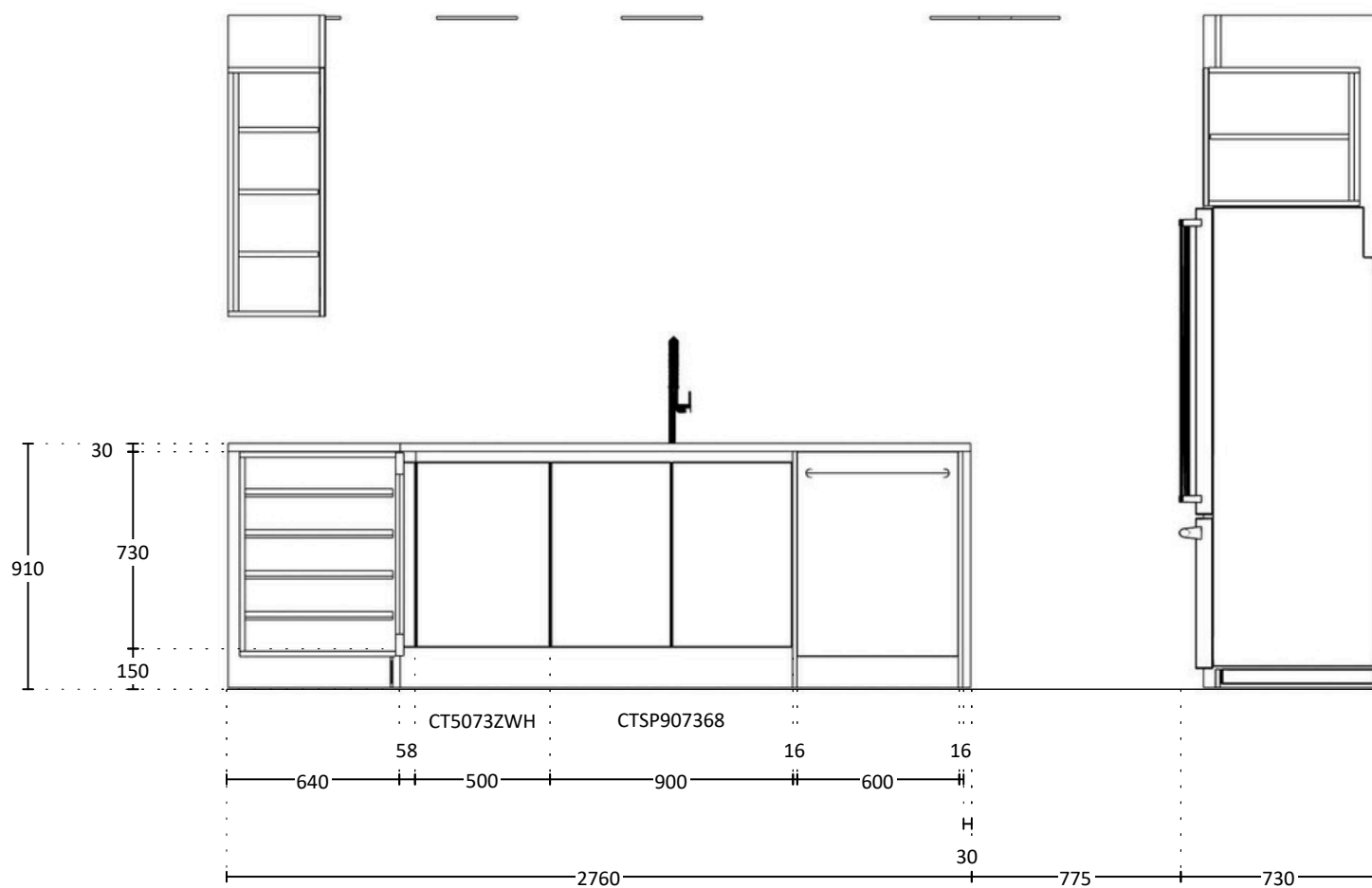
ELEVATION D
