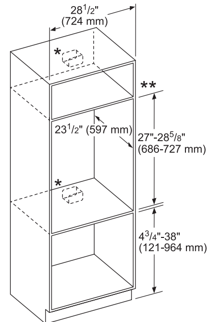
Single Oven Wall Mount Installation
