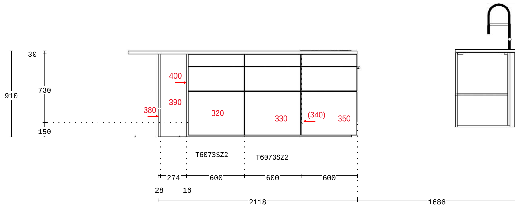
ELEVATION D
