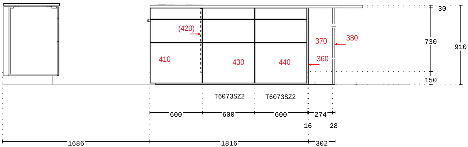
ELEVATION F
